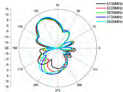
Three Ports in V-plane Cut-2
