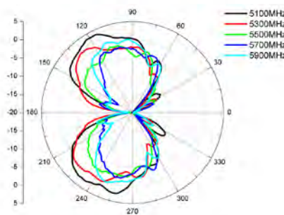
Three Ports in V-plane Cut-1
