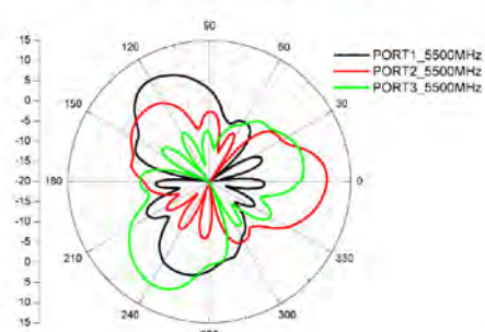
Three Ports in V-plane Cut-2
