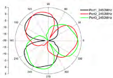
Three Ports in V-plane Cut-1
